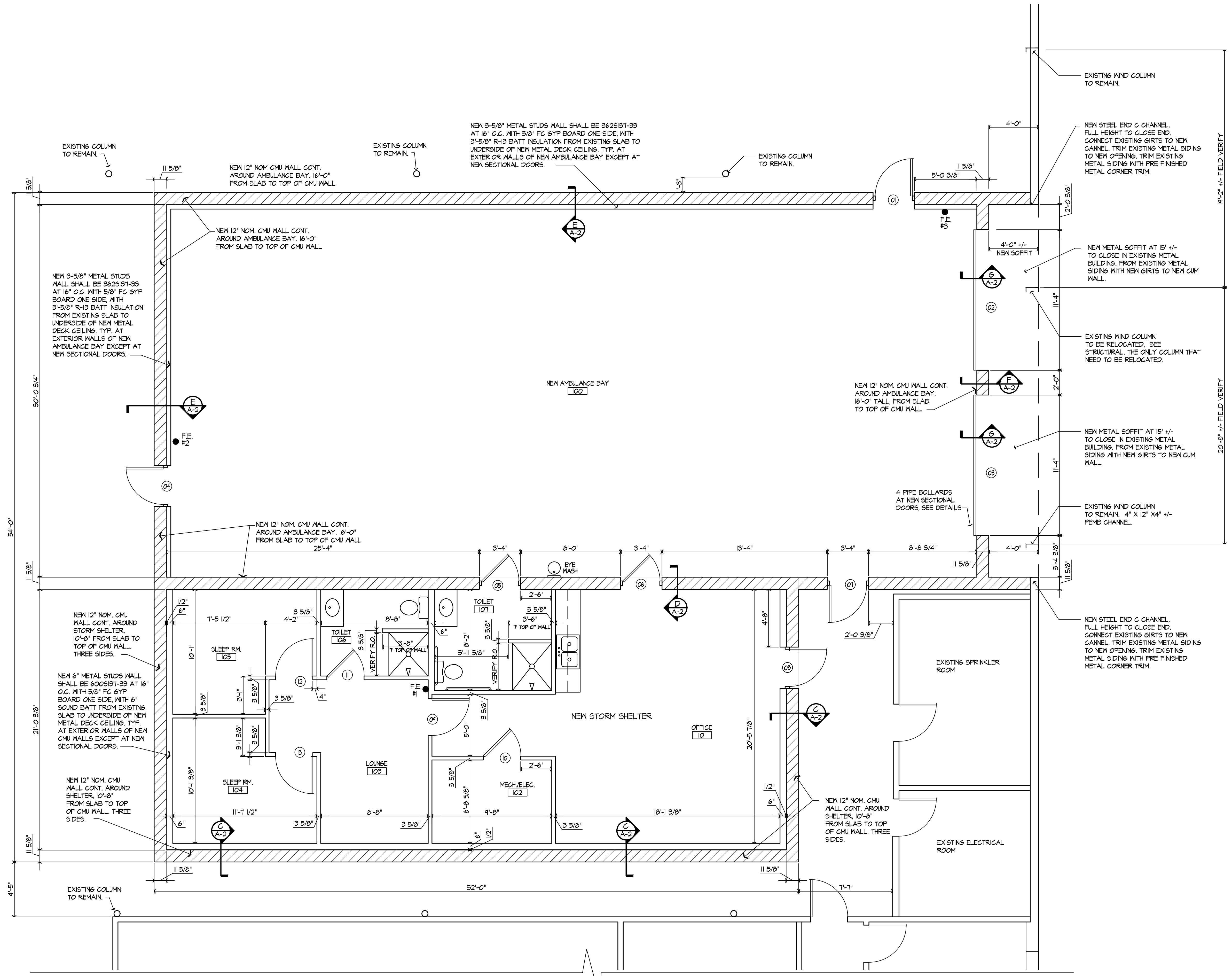
FLOOR PLAN SCALE: 1/4" = 1'-0" (A-A-1)
